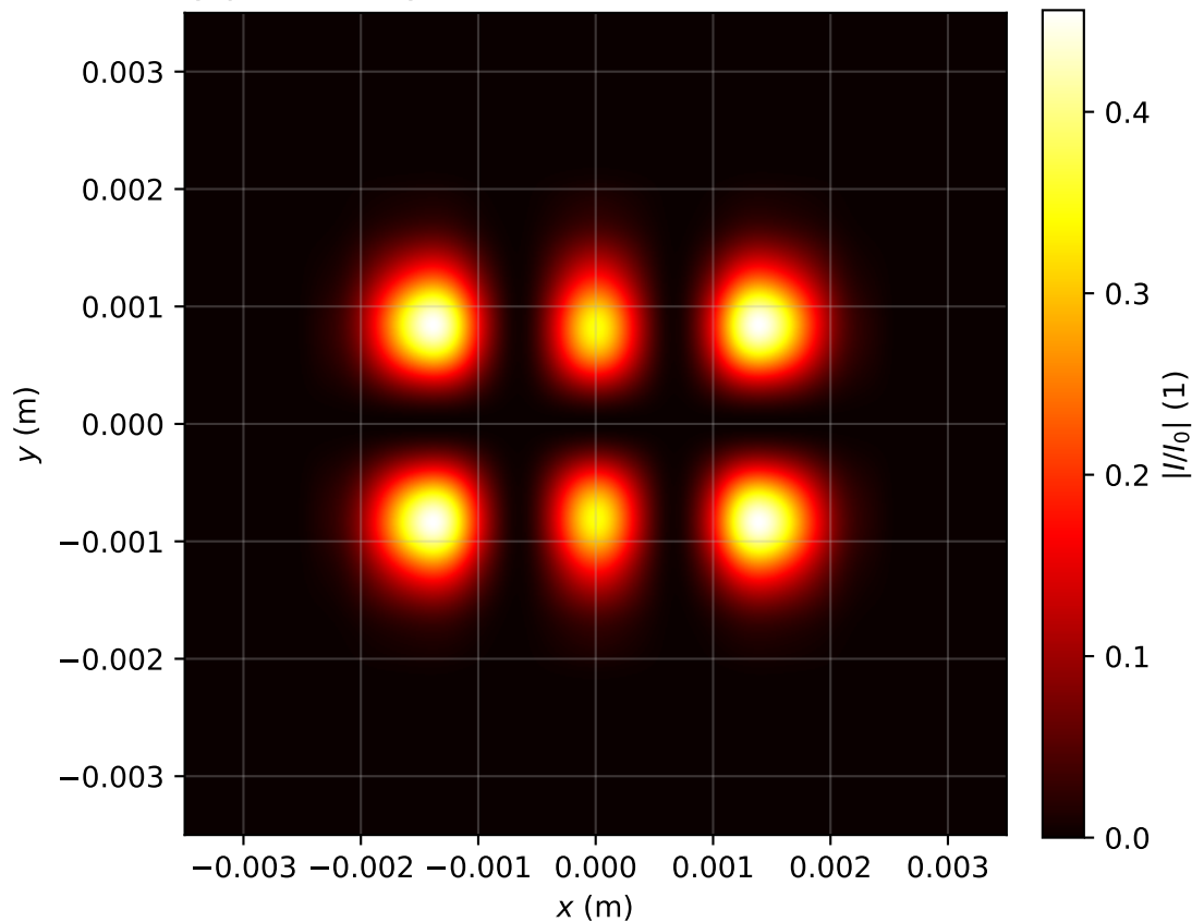
Intensity profile I(x, y, z = 2.946)/I_0 , P_{in}=2.0P_{cr} , artificial time
